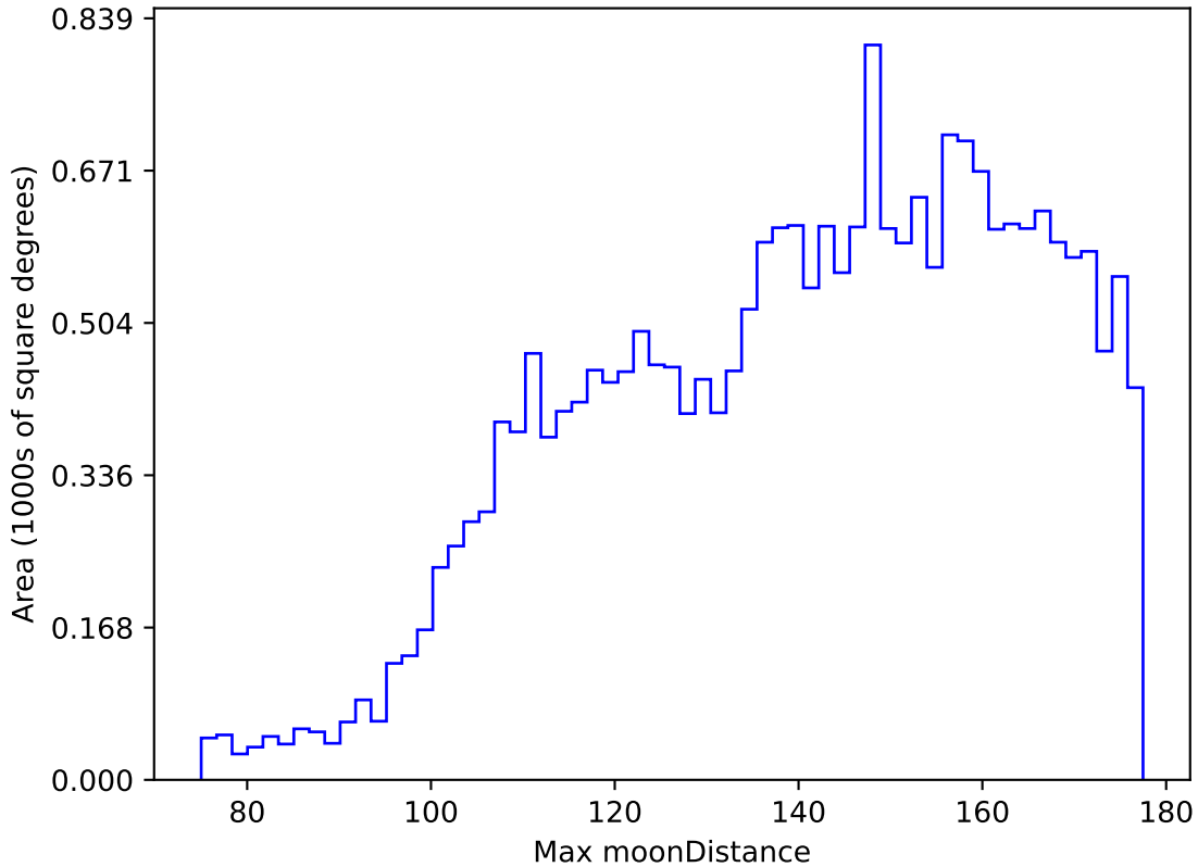
too_elab_r32_d3_gz_v3.4_10yrs All sky y band: Max moonDistance
