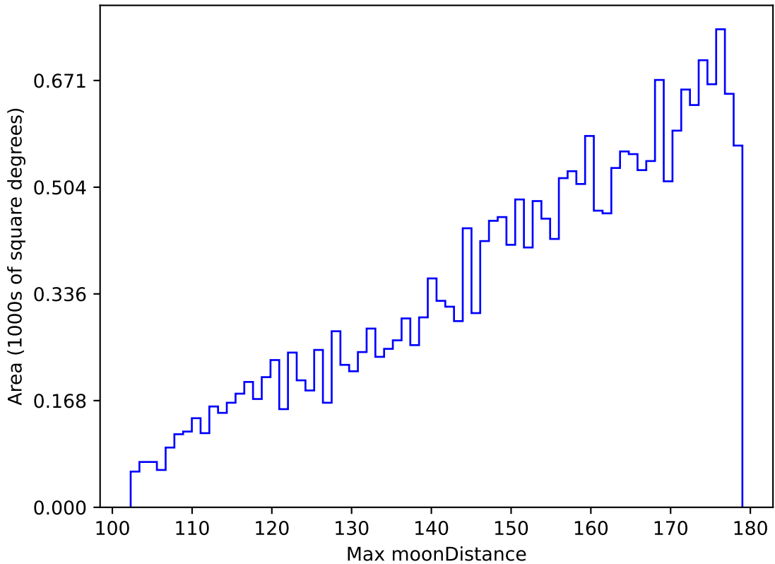
too_elab_r32_d3_gz_v3.4_10yrs All sky u band: Max moonDistance
