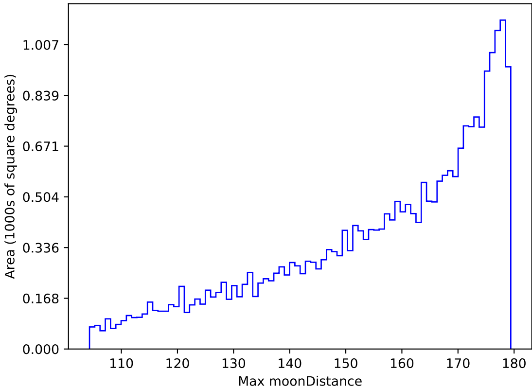
too_elab_r32_d3_gz_v3.4_10yrs All sky r band: Max moonDistance
