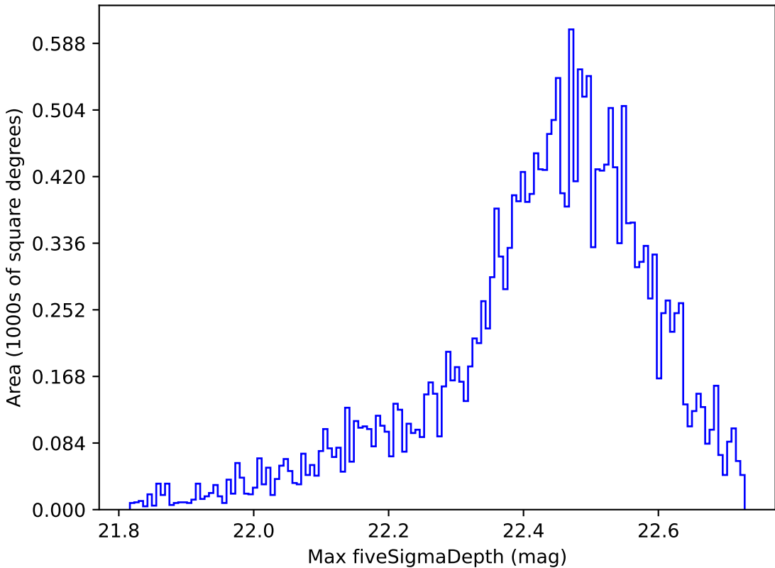
too_elab_r32_d3_gz_v3.4_10yrs Yr 1 y band: Max fiveSigmaDepth
