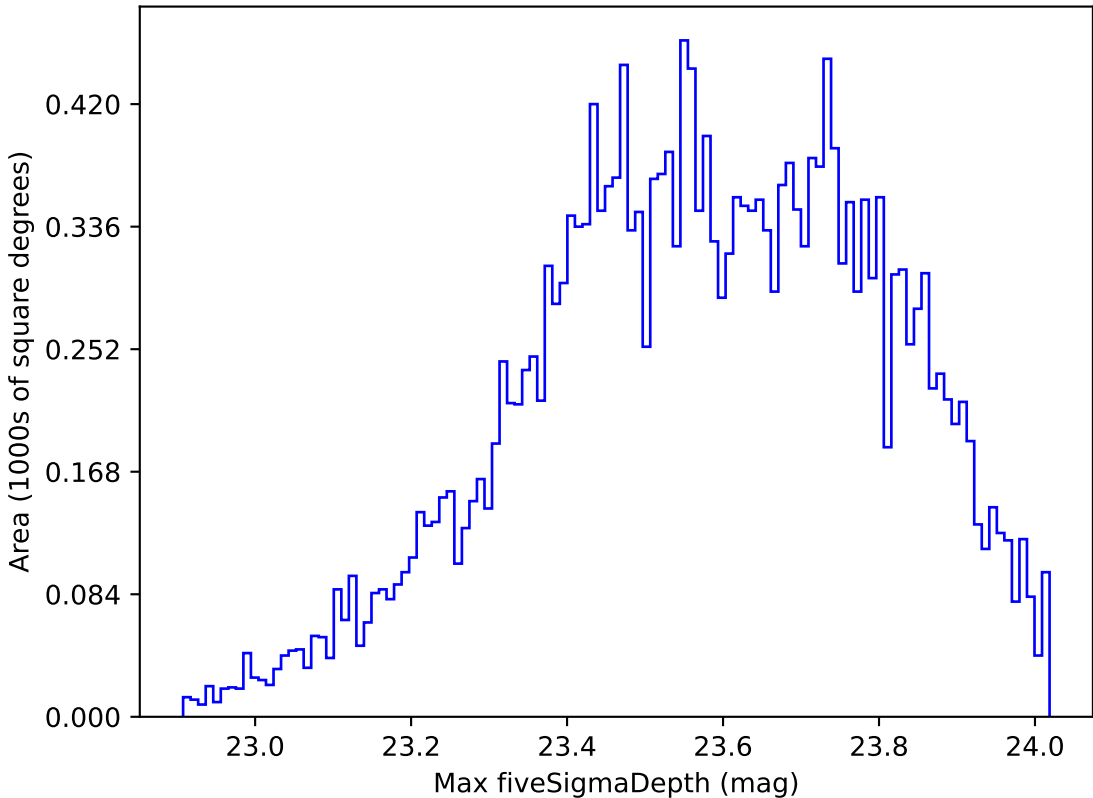
too_elab_r32_d3_gz_v3.4_10yrs Yr 1 u band: Max fiveSigmaDepth
