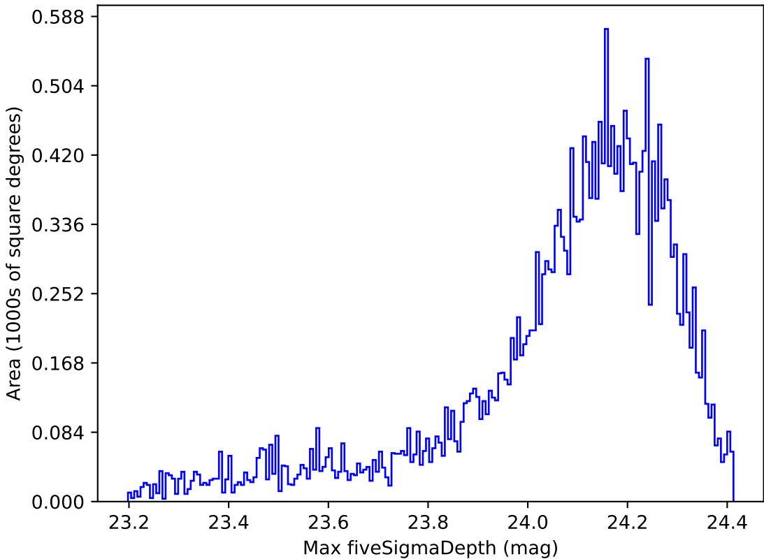
too_elab_r32_d3_gz_v3.4_10yrs Yr 1 i band: Max fiveSigmaDepth
