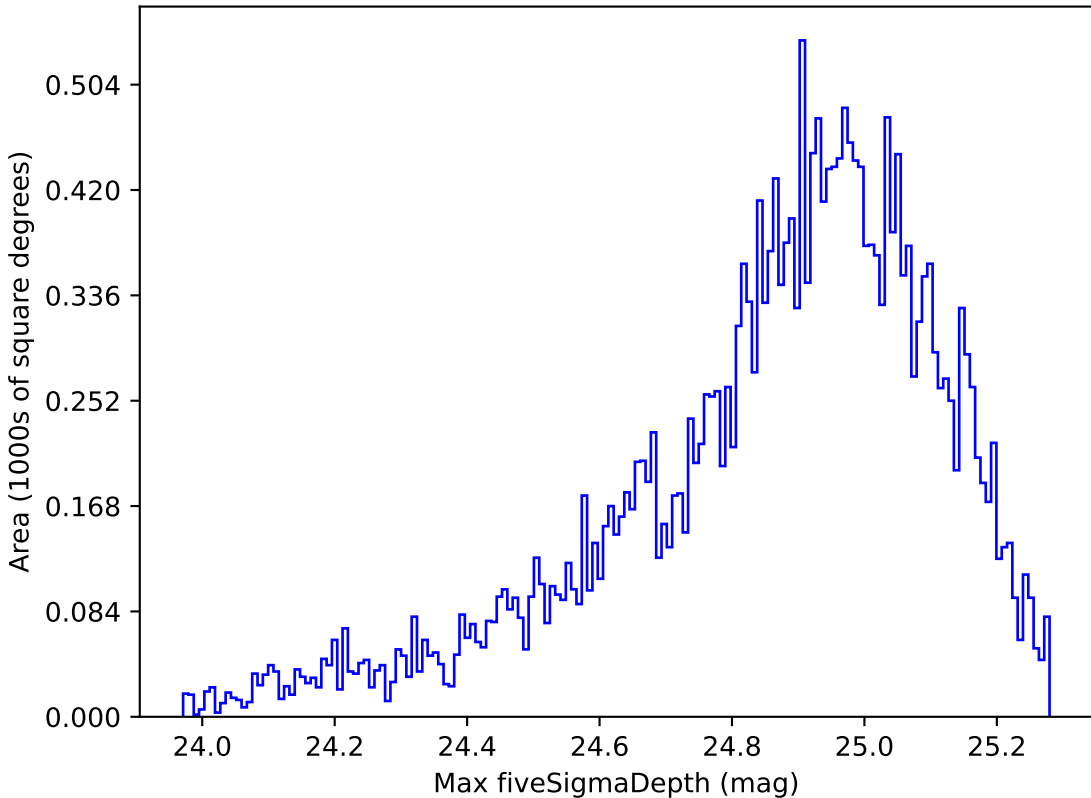
too_elab_r32_d3_gz_v3.4_10yrs Yr 1 g band: Max fiveSigmaDepth
