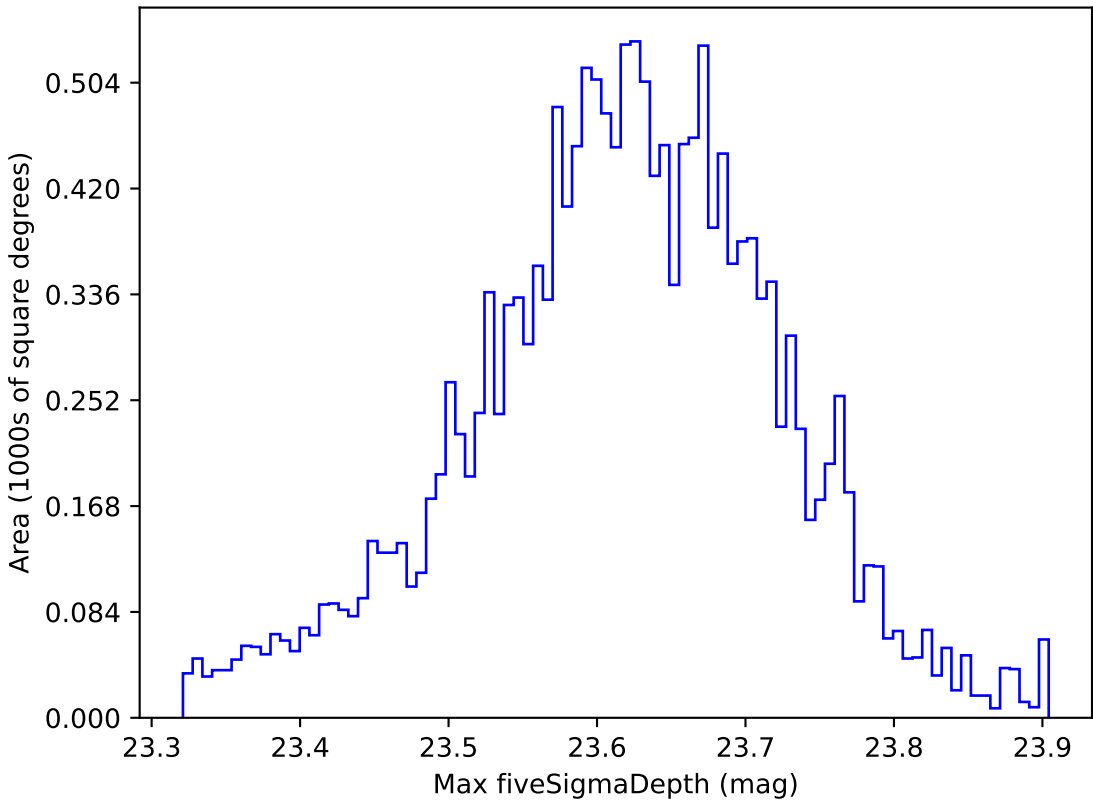
too_elab_r32_d3_gz_v3.4_10yrs WFD z band: Max fiveSigmaDepth
