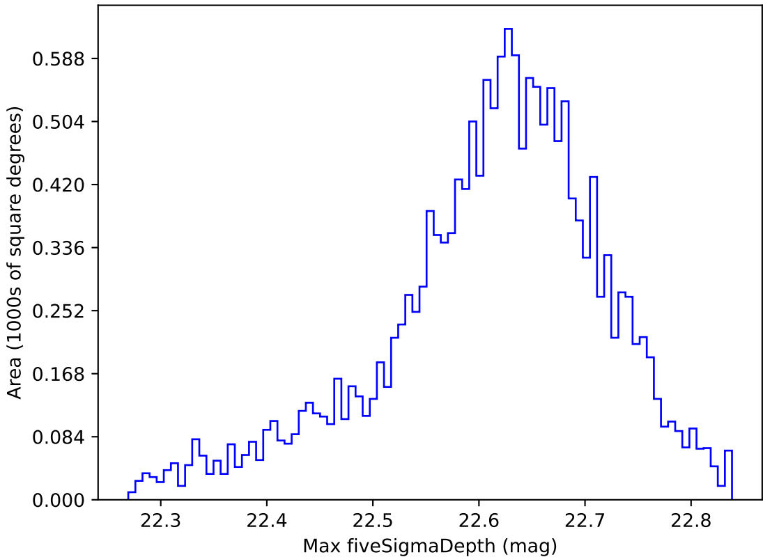
too_elab_r32_d3_gz_v3.4_10yrs WFD y band: Max fiveSigmaDepth
