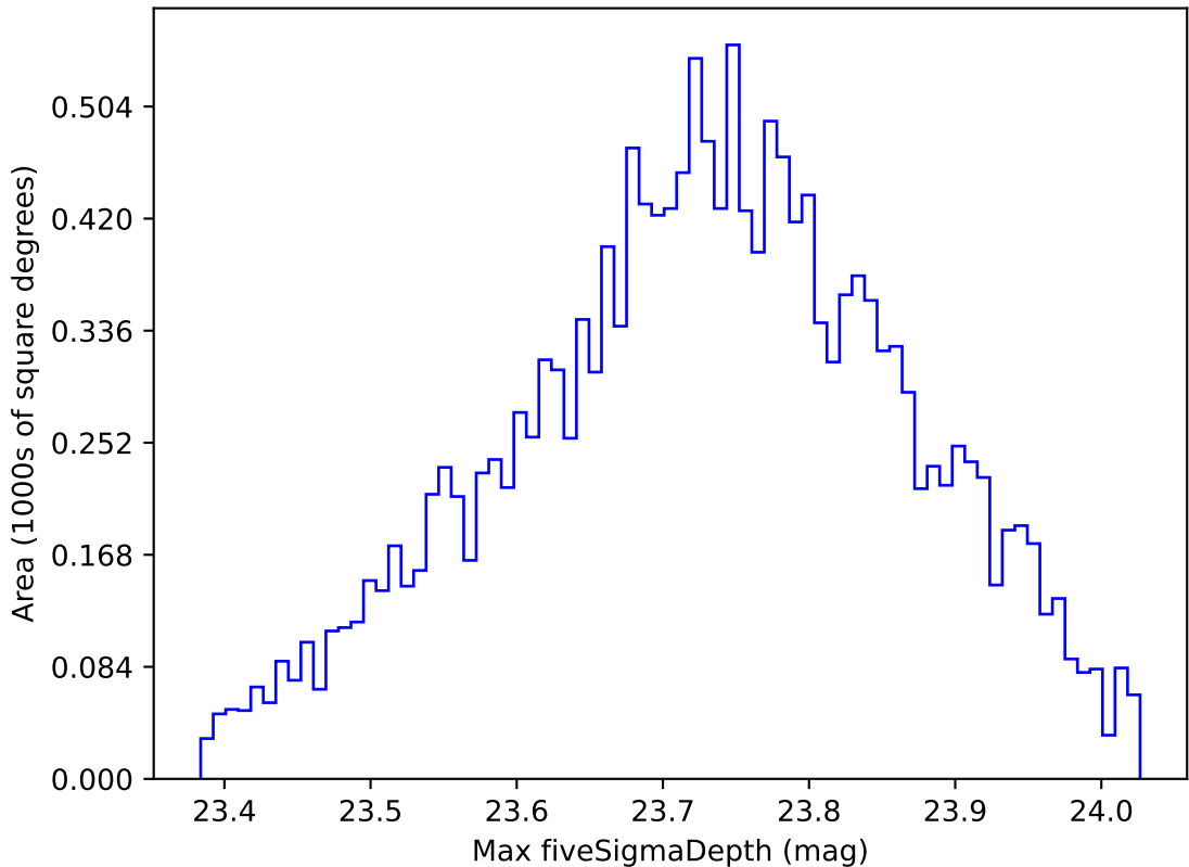
too_elab_r32_d3_gz_v3.4_10yrs WFD u band: Max fiveSigmaDepth
