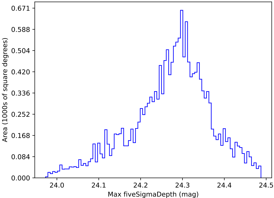
too_elab_r32_d3_gz_v3.4_10yrs WFD i band: Max fiveSigmaDepth
