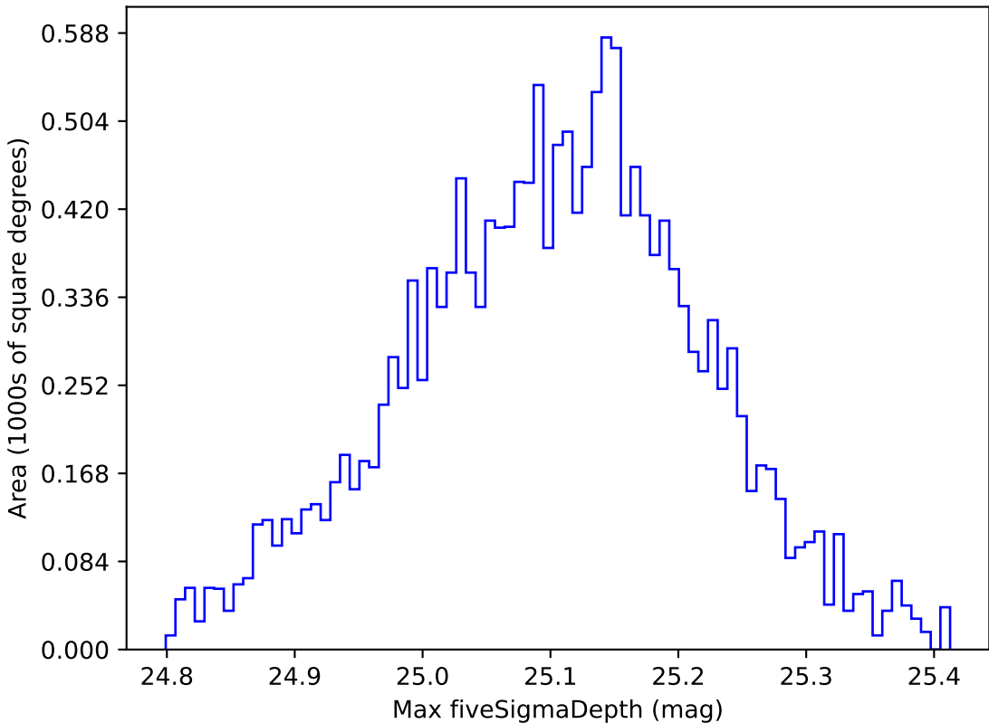
too_elab_r32_d3_gz_v3.4_10yrs WFD all bands: Max fiveSigmaDepth
