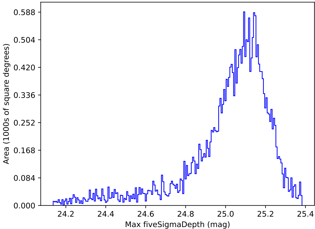
too_elab_r32_d3_gz_v3.4_10yrs All sky g band: Max fiveSigmaDepth
