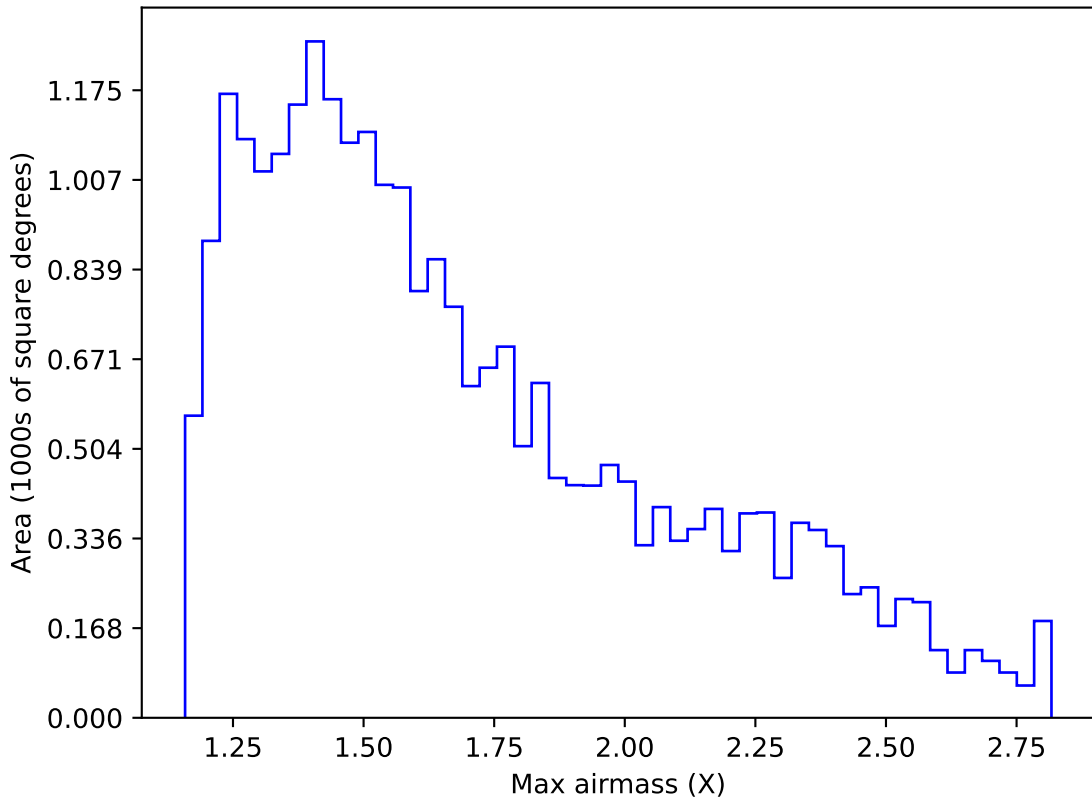
too_elab_r32_d3_gz_v3.4_10yrs Yr 1 z band: Max airmass
