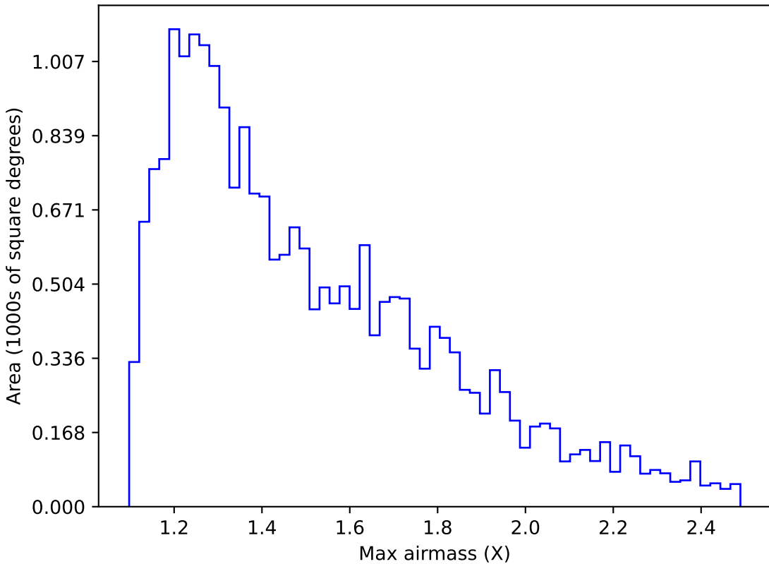
too_elab_r32_d3_gz_v3.4_10yrs Yr 1 u band: Max airmass
