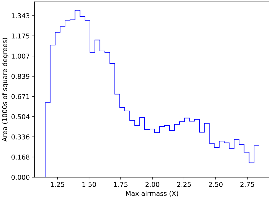
too_elab_r32_d3_gz_v3.4_10yrs Yr 1 i band: Max airmass
