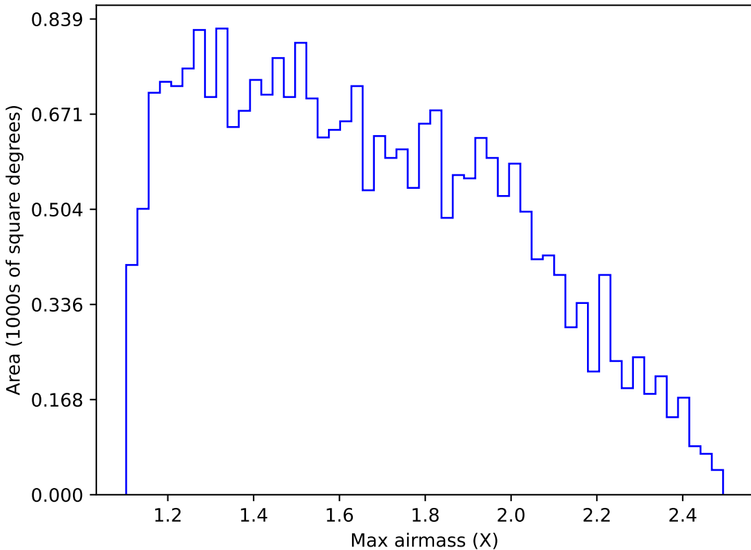
too_elab_r32_d3_gz_v3.4_10yrs Yr 1 g band: Max airmass
