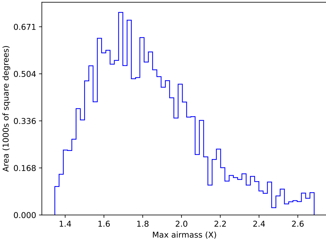
too_elab_r32_d3_gz_v3.4_10yrs WFD u band: Max airmass
