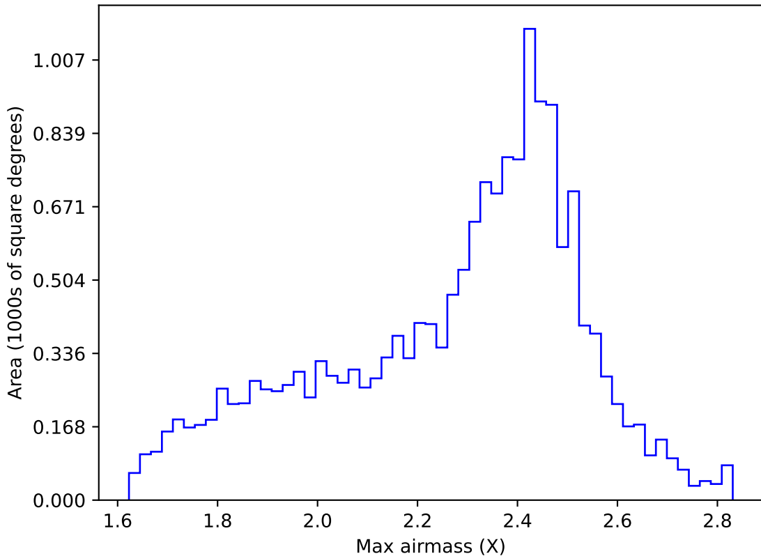
too_elab_r32_d3_gz_v3.4_10yrs WFD r band: Max airmass
