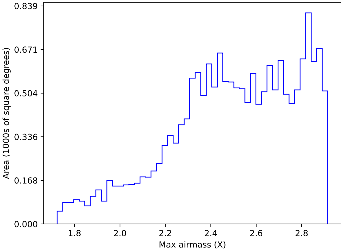
too_elab_r32_d3_gz_v3.4_10yrs WFD i band: Max airmass
