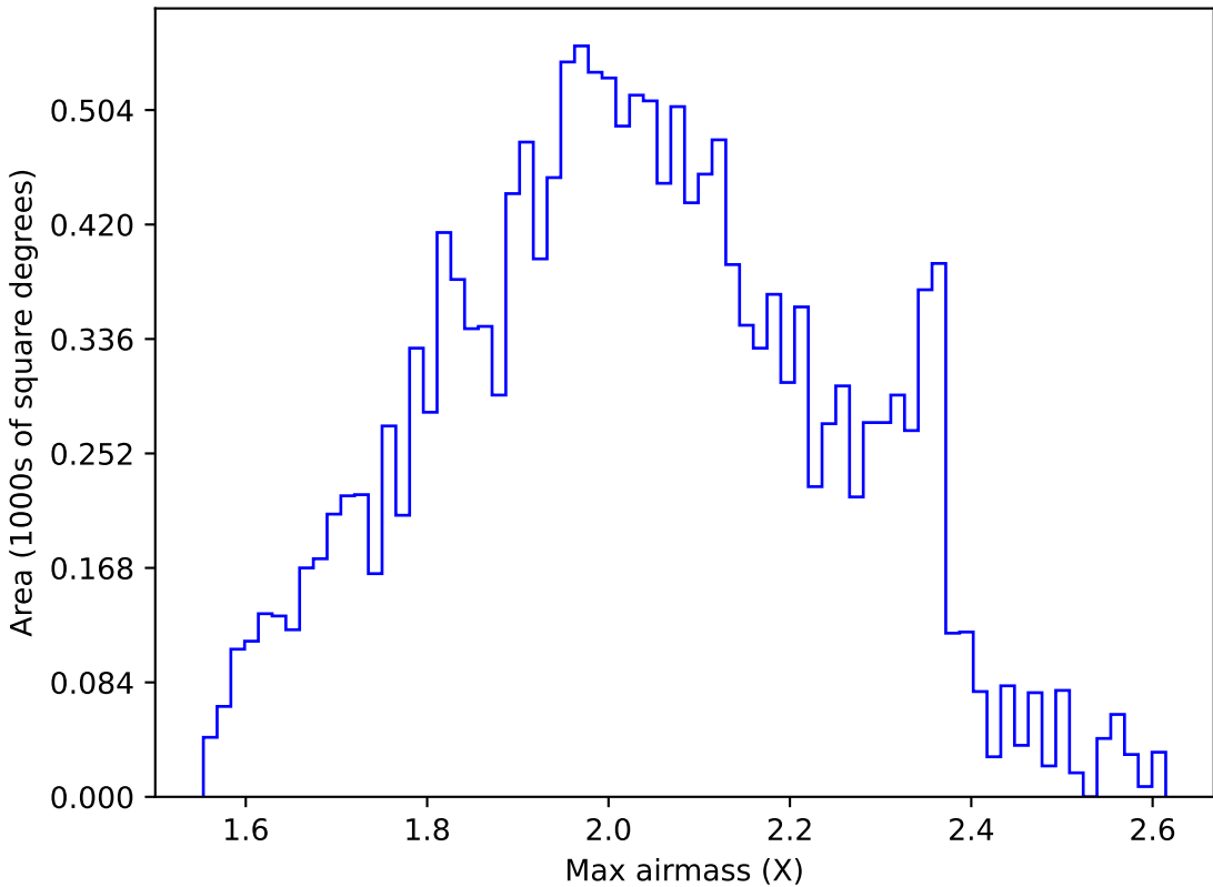
too_elab_r32_d3_gz_v3.4_10yrs WFD g band: Max airmass
