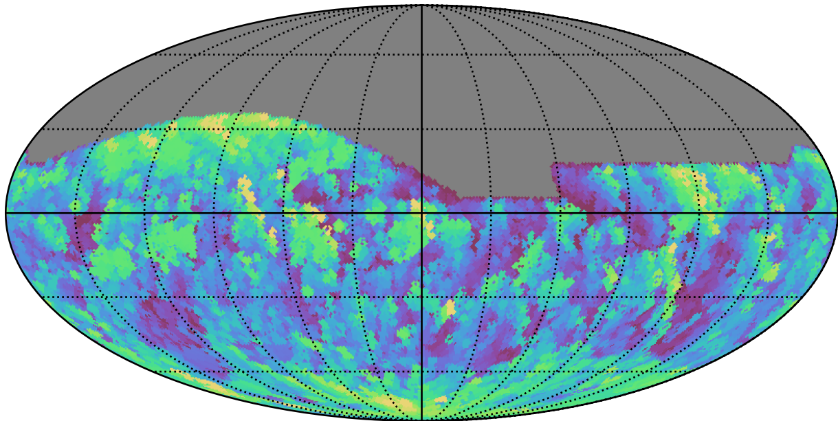
too_elab_r32_d3_gz_v3.4_10yrs All sky g band: Max airmass
