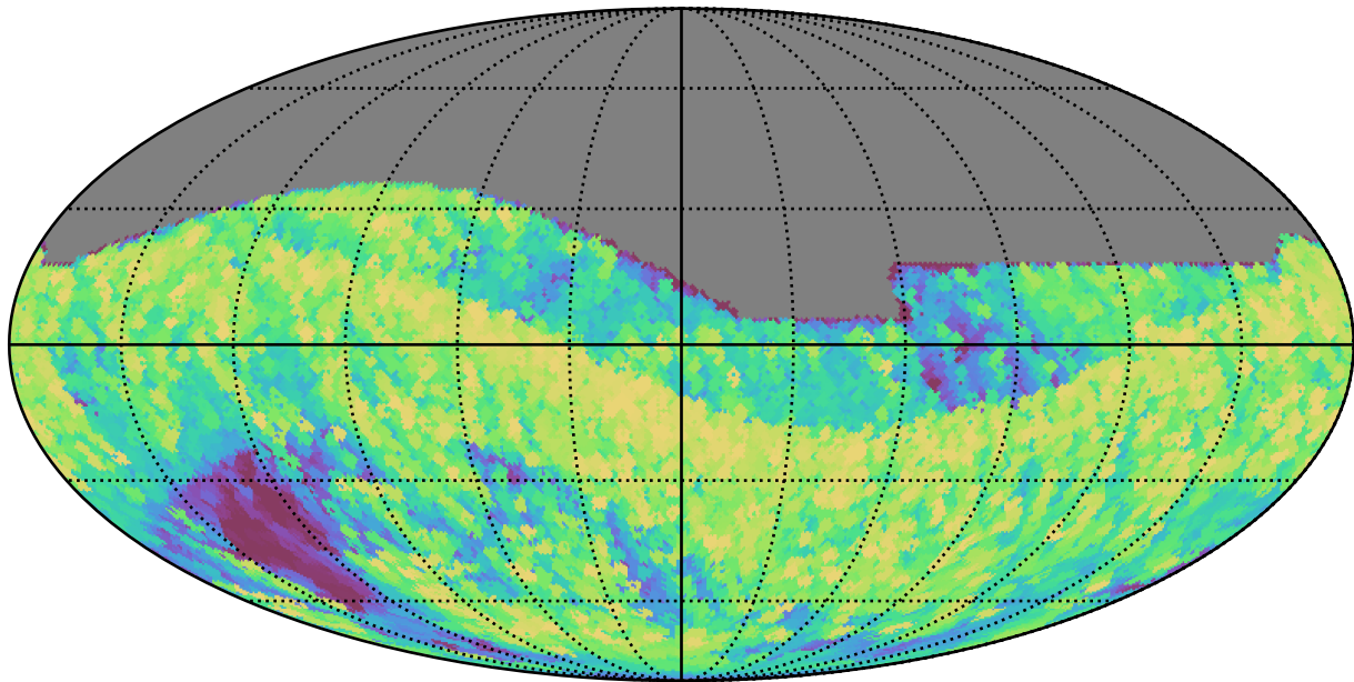
too_elab_r32_d3_gz_v3.4_10yrs All sky all bands: Max airmass
