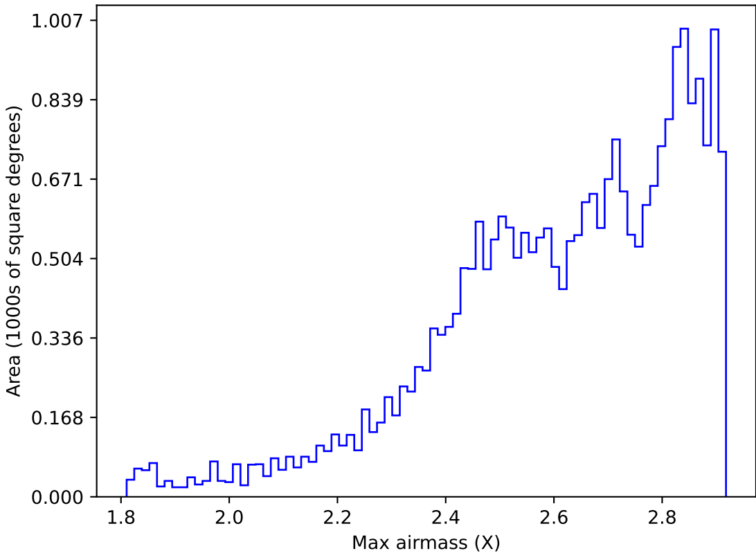
too_elab_r32_d3_gz_v3.4_10yrs All sky all bands: Max airmass
