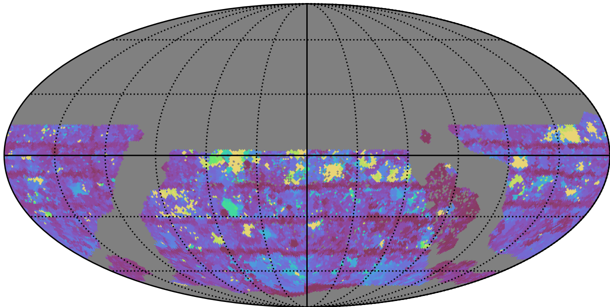
too_elab_r32_d3_gz_v3.4_10yrs WFD z band: Max Inter-Night Gap
