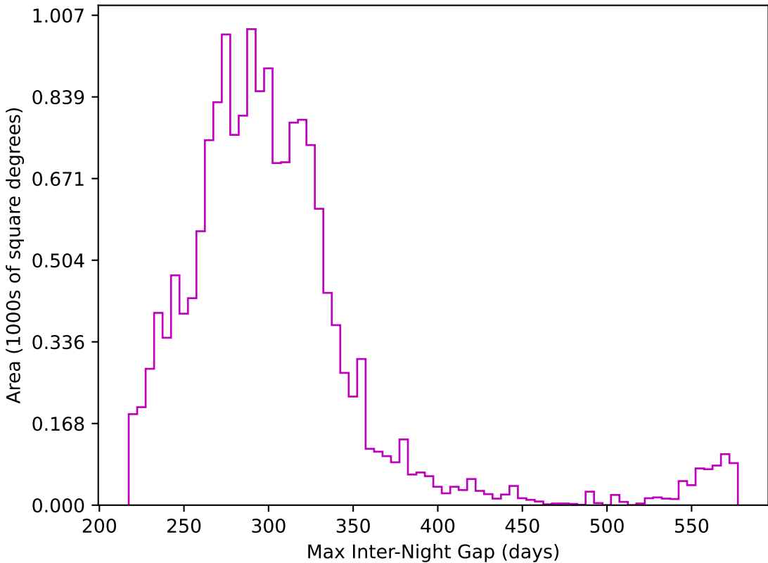
too_elab_r32_d3_gz_v3.4_10yrs WFD z band: Max Inter-Night Gap
