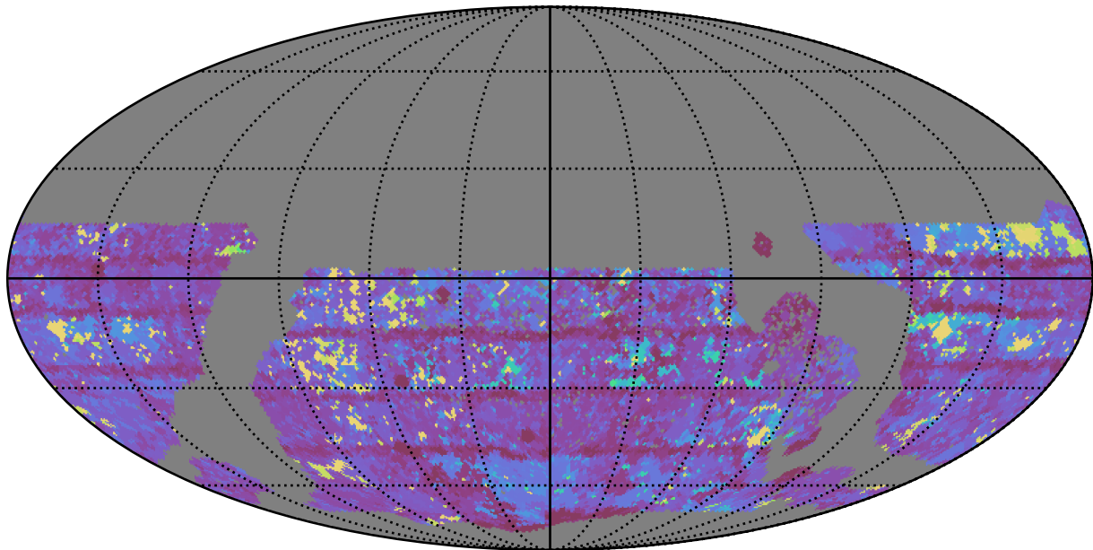
too_elab_r32_d3_gz_v3.4_10yrs WFD y band: Max Inter-Night Gap
