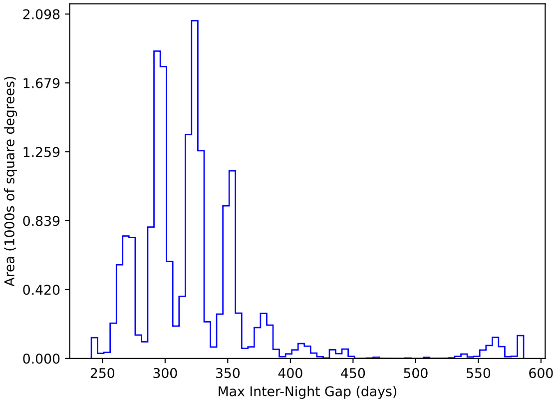
too_elab_r32_d3_gz_v3.4_10yrs WFD y band: Max Inter-Night Gap
