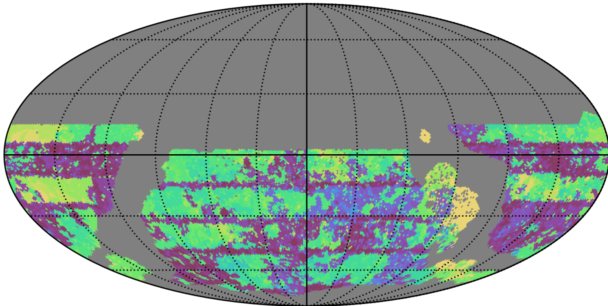
too_elab_r32_d3_gz_v3.4_10yrs WFD u band: Max Inter-Night Gap
