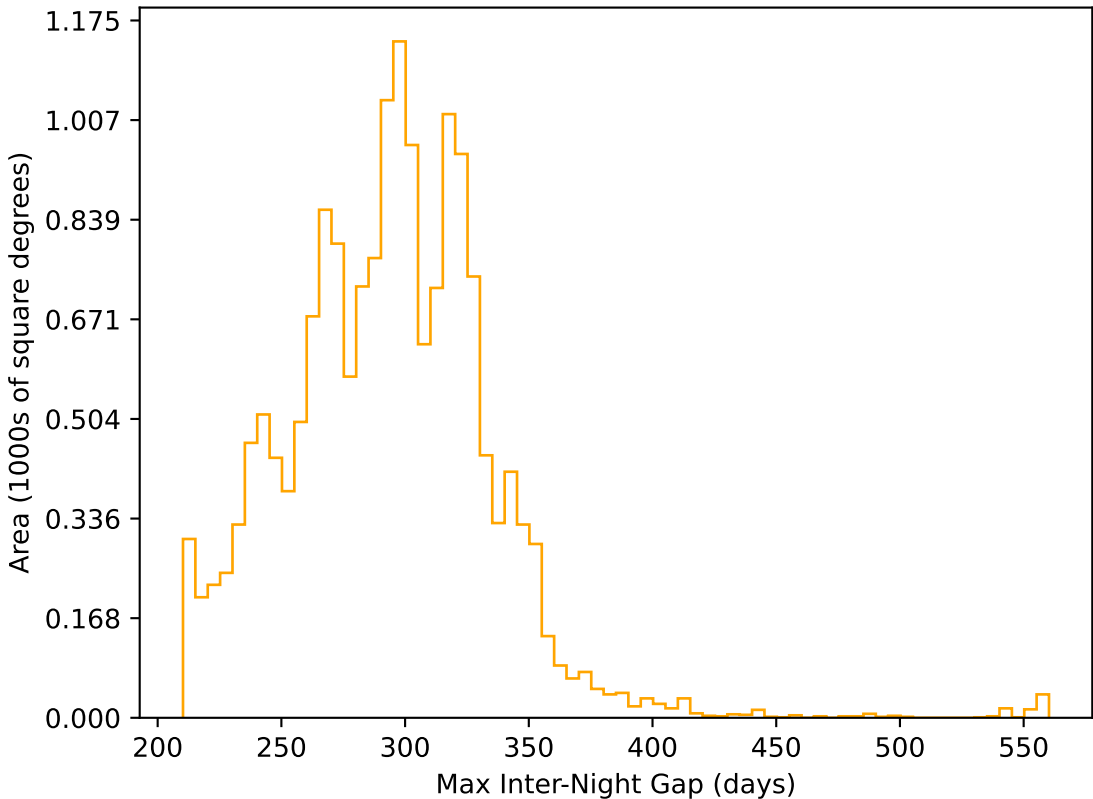
too_elab_r32_d3_gz_v3.4_10yrs WFD r band: Max Inter-Night Gap
