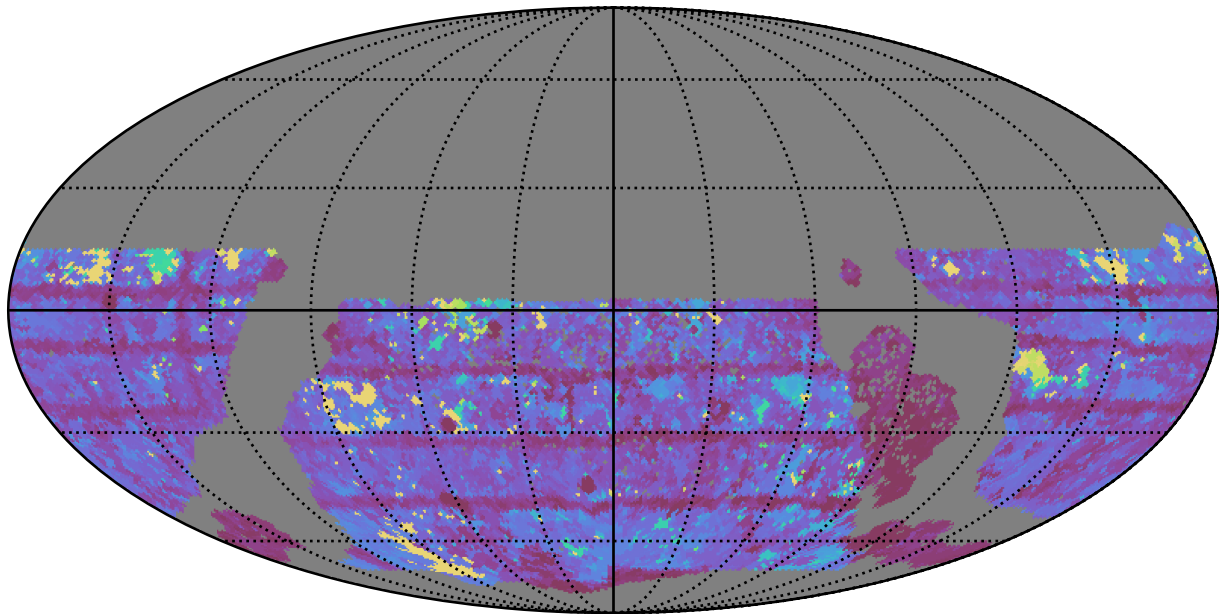
too_elab_r32_d3_gz_v3.4_10yrs WFD i band: Max Inter-Night Gap
