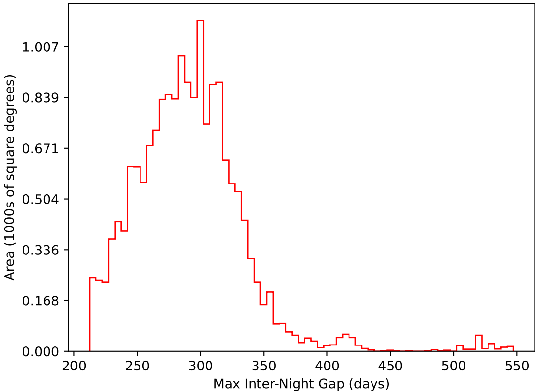
too_elab_r32_d3_gz_v3.4_10yrs WFD i band: Max Inter-Night Gap
