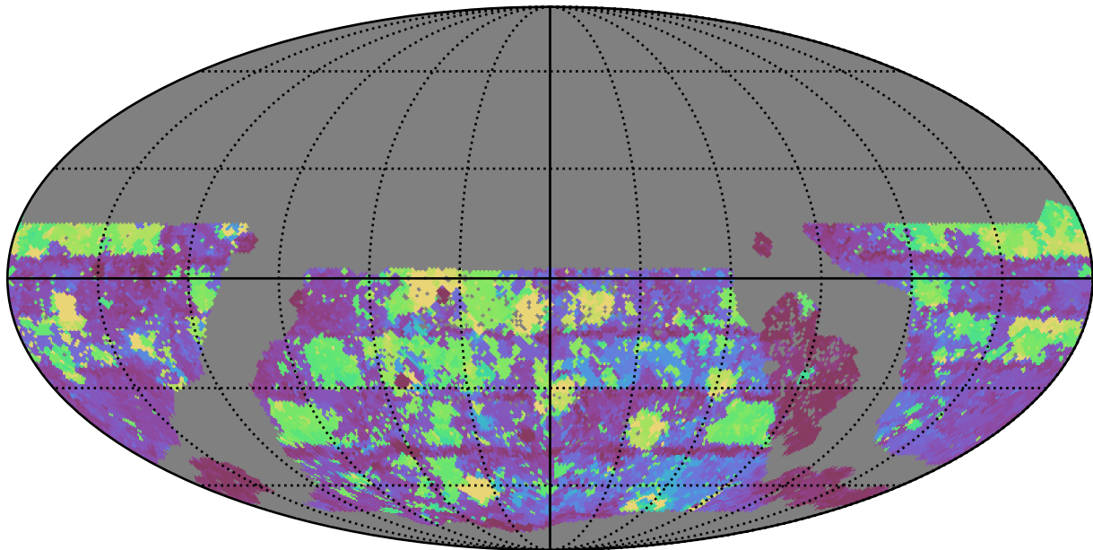
too_elab_r32_d3_gz_v3.4_10yrs WFD g band: Max Inter-Night Gap
