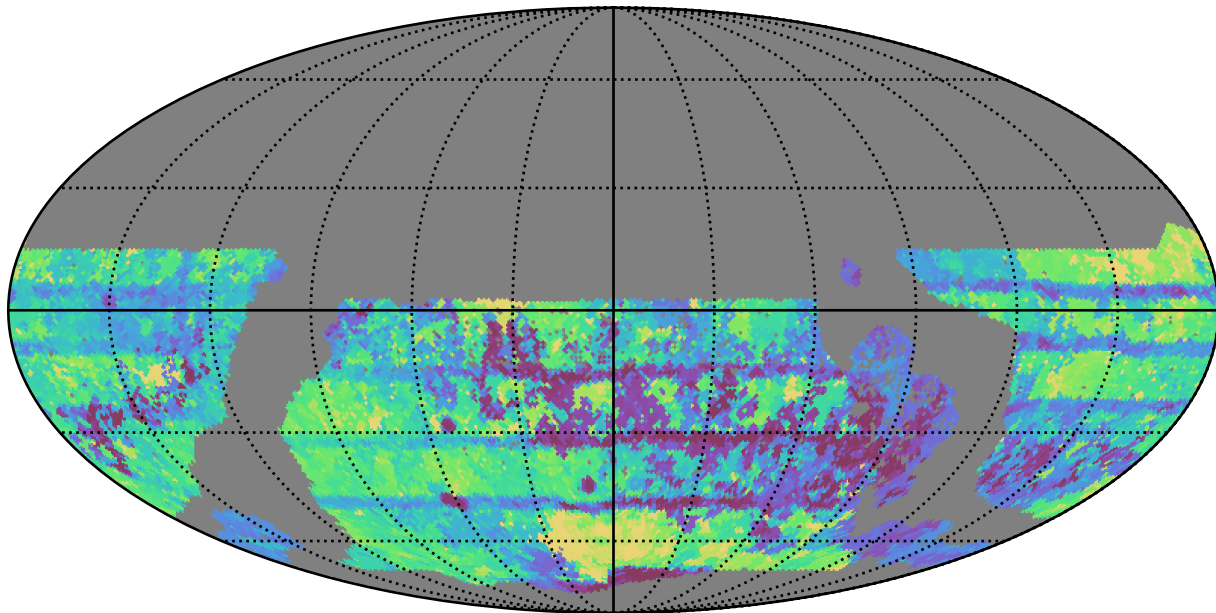
too_elab_r32_d3_gz_v3.4_10yrs WFD all bands: Max Inter-Night Gap
