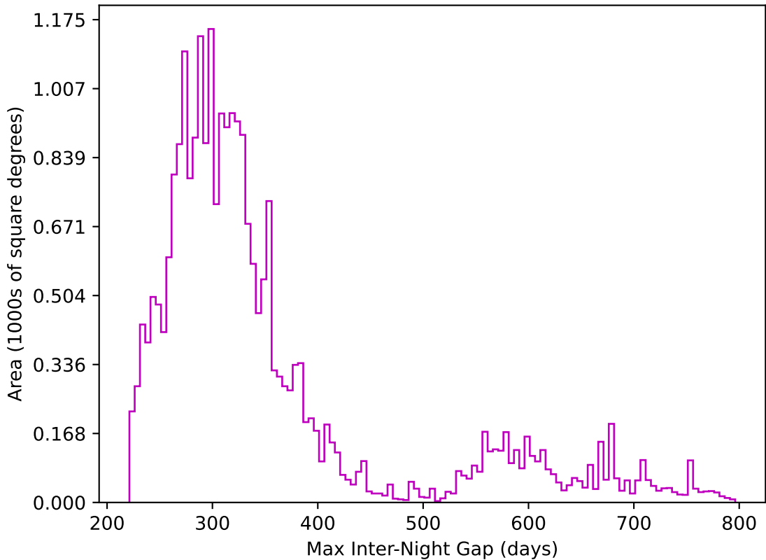
too_elab_r32_d3_gz_v3.4_10yrs All sky z band: Max Inter-Night Gap
