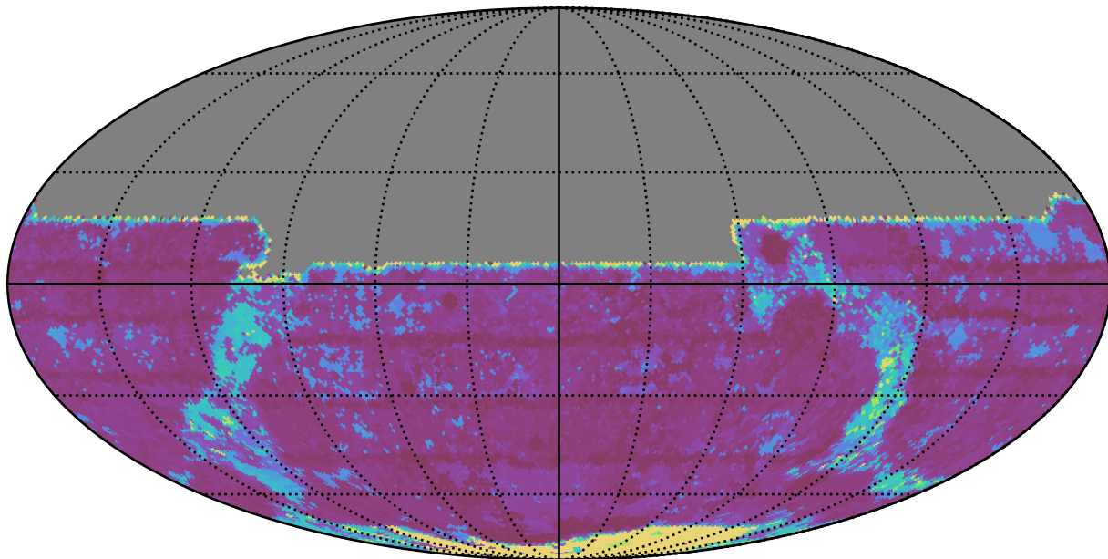
too_elab_r32_d3_gz_v3.4_10yrs All sky y band: Max Inter-Night Gap
