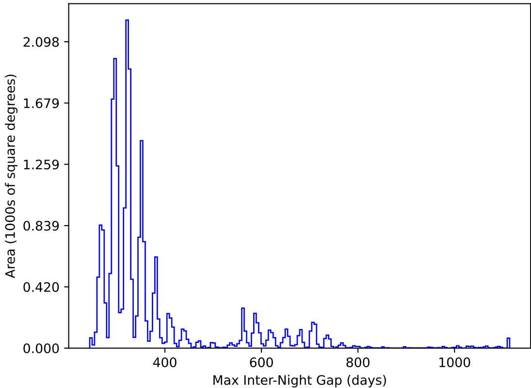
too_elab_r32_d3_gz_v3.4_10yrs All sky y band: Max Inter-Night Gap
