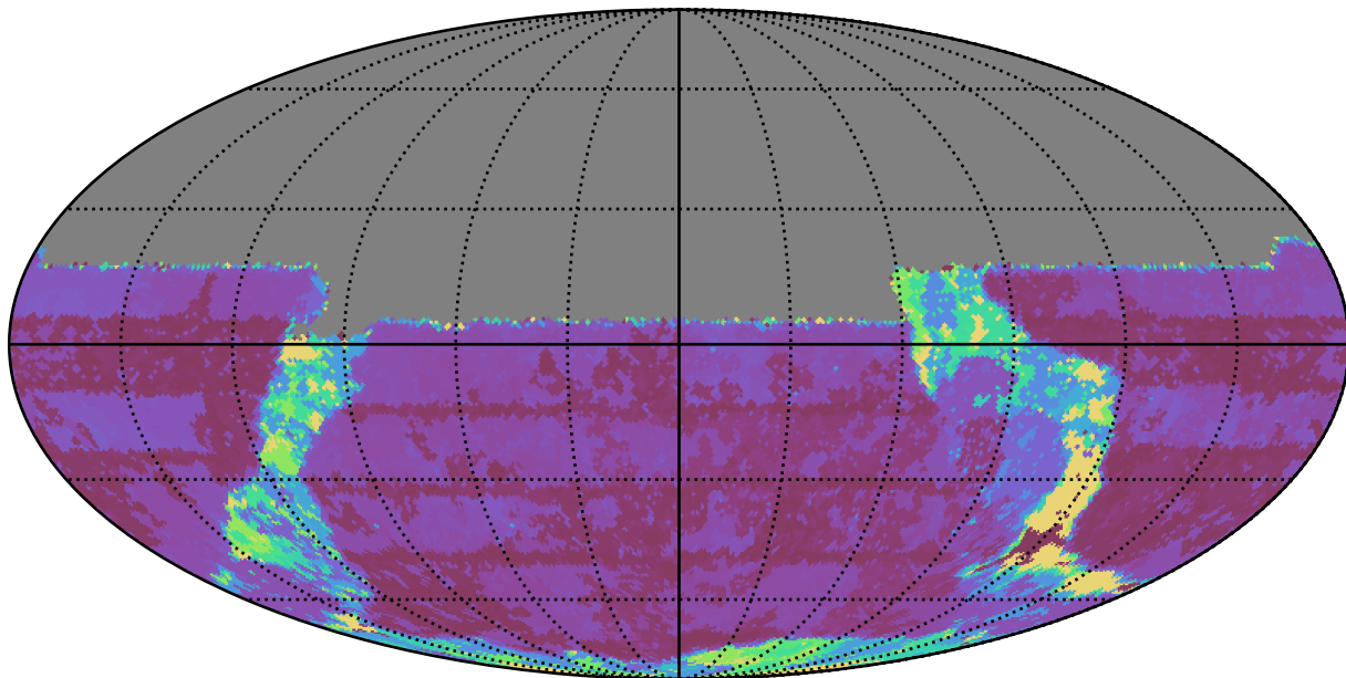
too_elab_r32_d3_gz_v3.4_10yrs All sky u band: Max Inter-Night Gap
