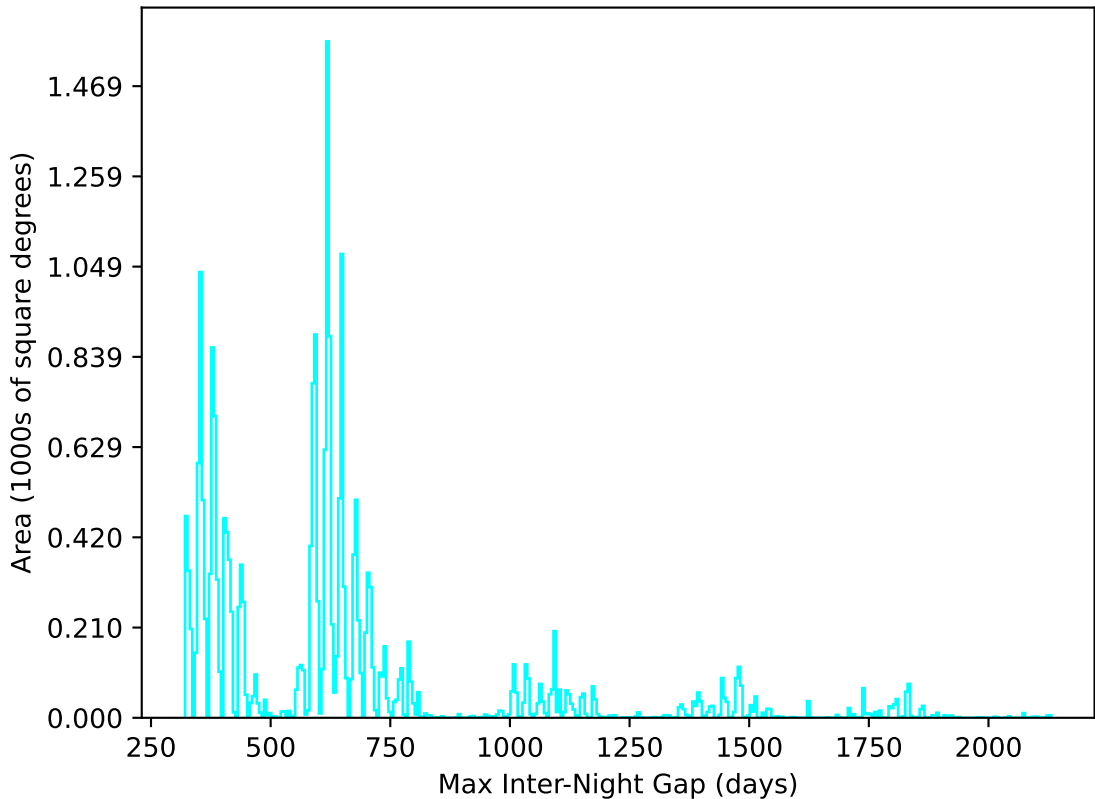
too_elab_r32_d3_gz_v3.4_10yrs All sky u band: Max Inter-Night Gap
