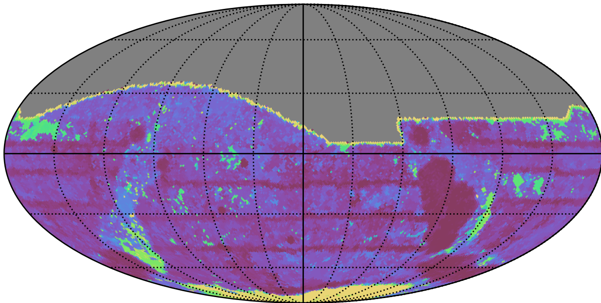
too_elab_r32_d3_gz_v3.4_10yrs All sky r band: Max Inter-Night Gap
