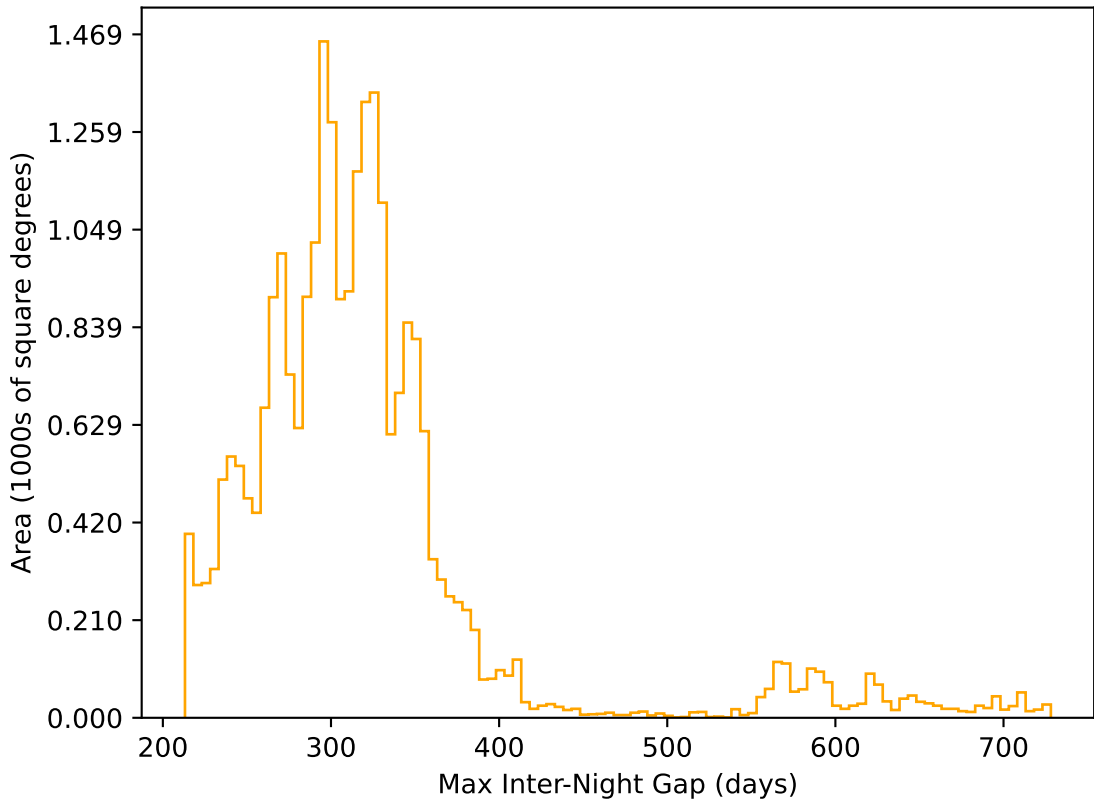
too_elab_r32_d3_gz_v3.4_10yrs All sky r band: Max Inter-Night Gap
