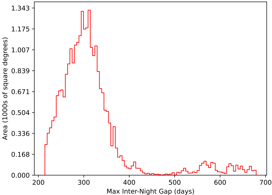
too_elab_r32_d3_gz_v3.4_10yrs All sky i band: Max Inter-Night Gap
