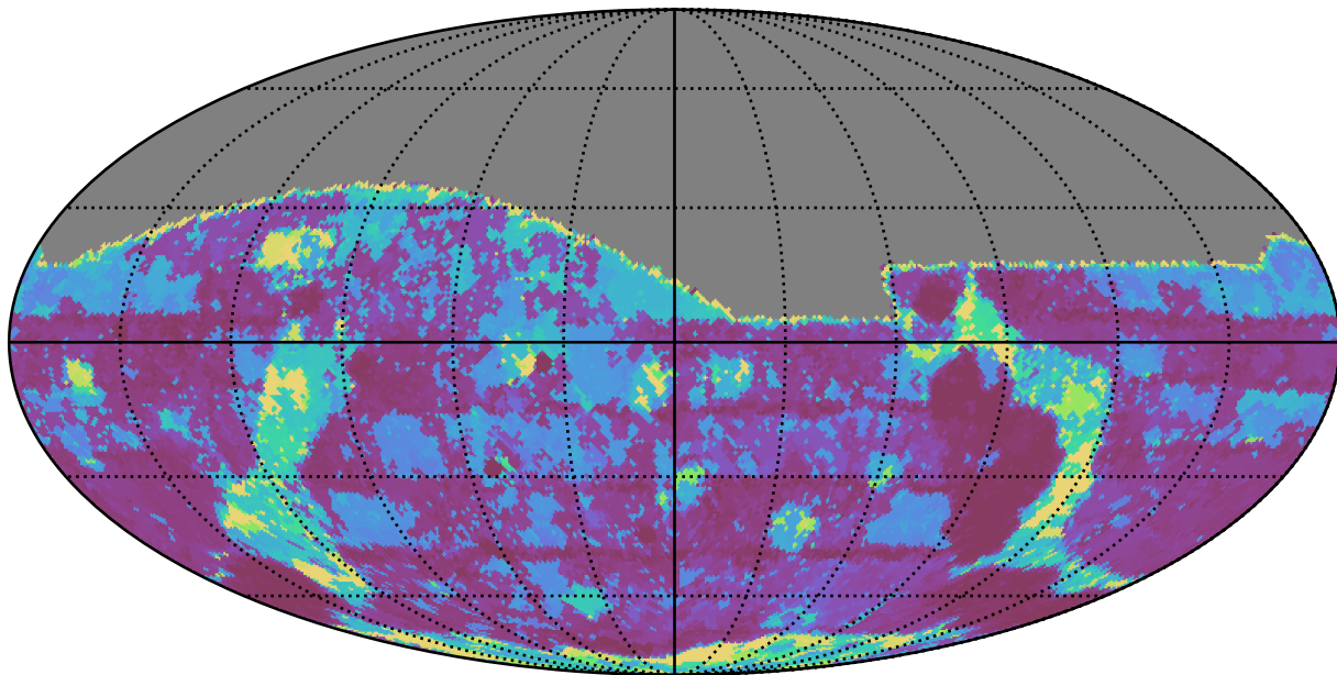
too_elab_r32_d3_gz_v3.4_10yrs All sky g band: Max Inter-Night Gap
