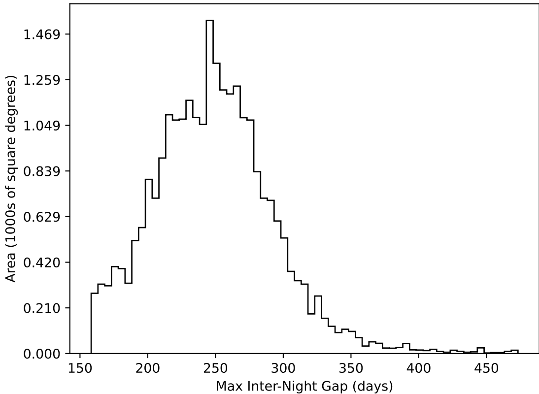
too_elab_r32_d3_gz_v3.4_10yrs All sky all bands: Max Inter-Night Gap
