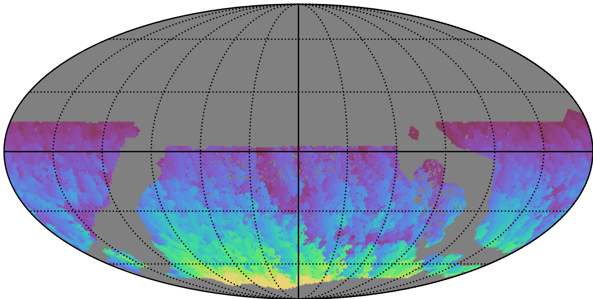
too_elab_r32_d3_gz_v3.4_10yrs WFD y band: Max HA
