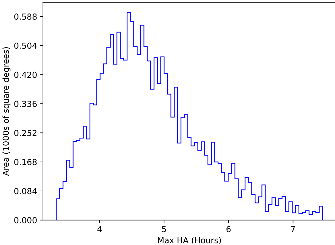
too_elab_r32_d3_gz_v3.4_10yrs WFD y band: Max HA
