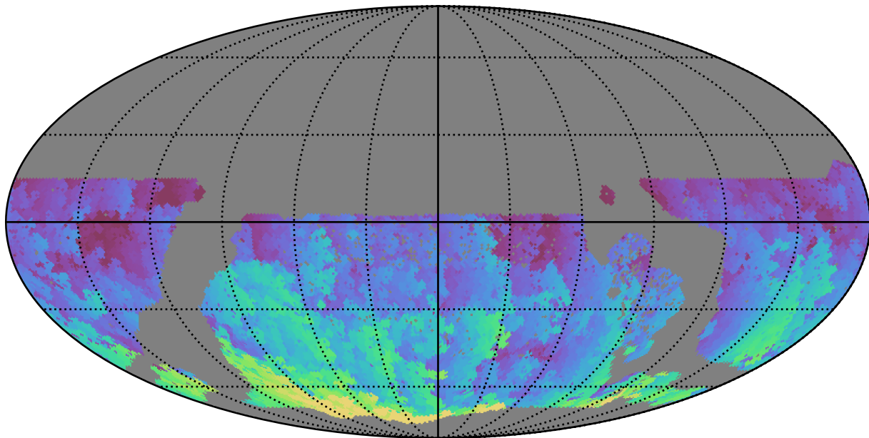
too_elab_r32_d3_gz_v3.4_10yrs WFD u band: Max HA
