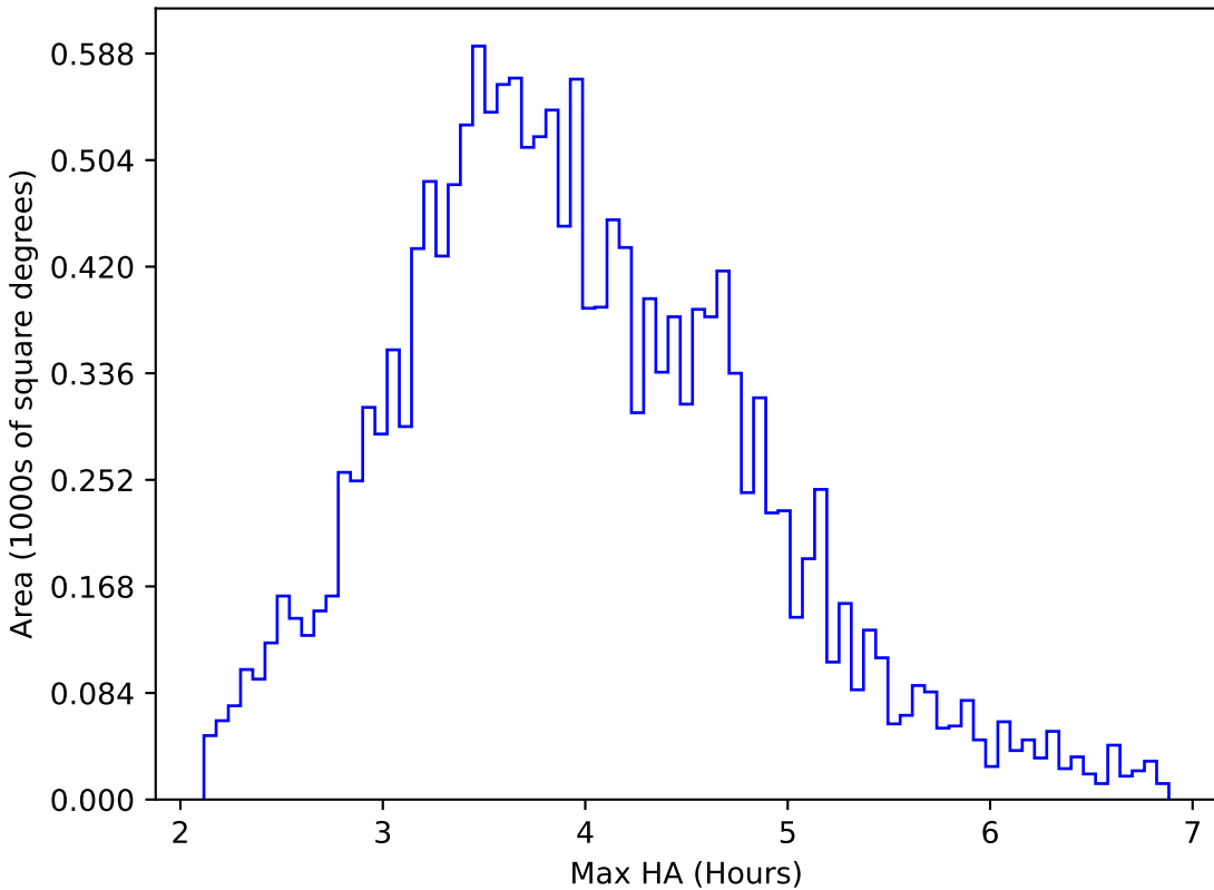
too_elab_r32_d3_gz_v3.4_10yrs WFD u band: Max HA
