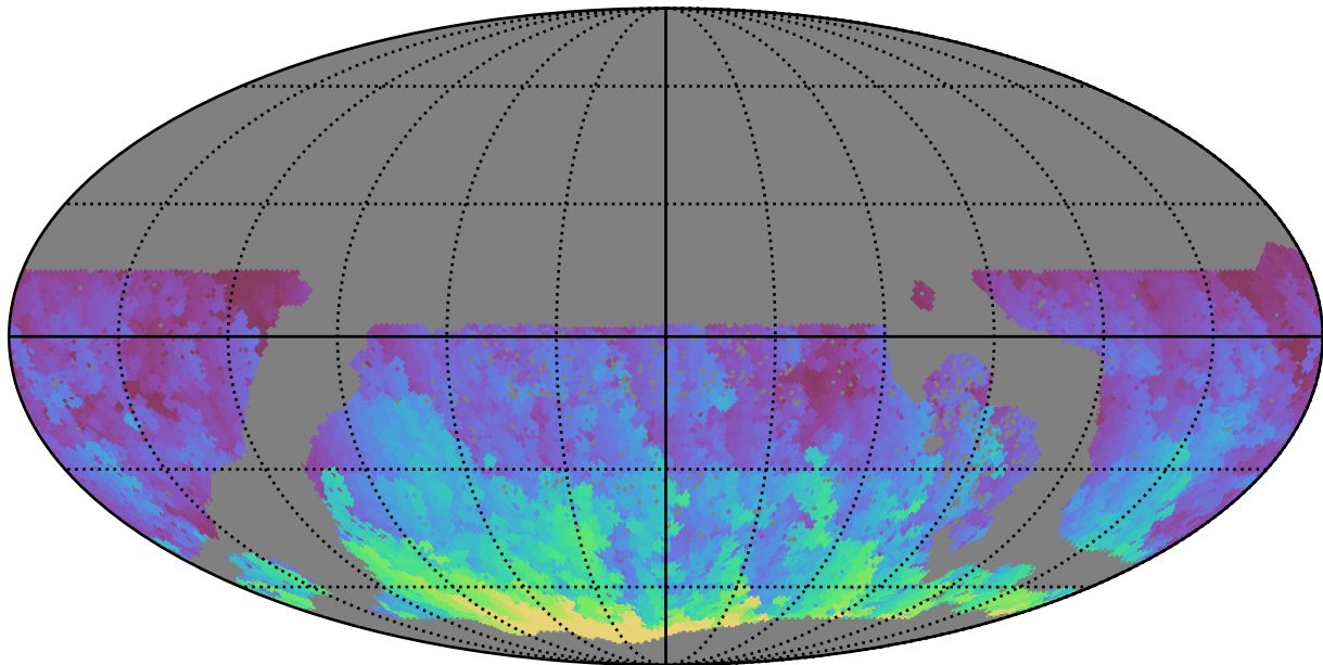
too_elab_r32_d3_gz_v3.4_10yrs WFD r band: Max HA
