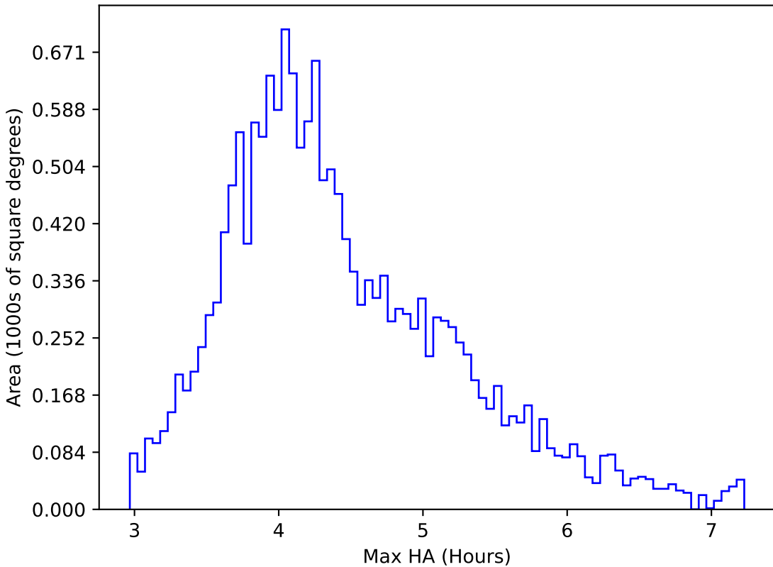
too_elab_r32_d3_gz_v3.4_10yrs WFD r band: Max HA
